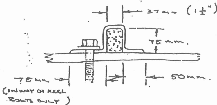
SECTION OF FLOORWEBS IN WAY OF KEEL
